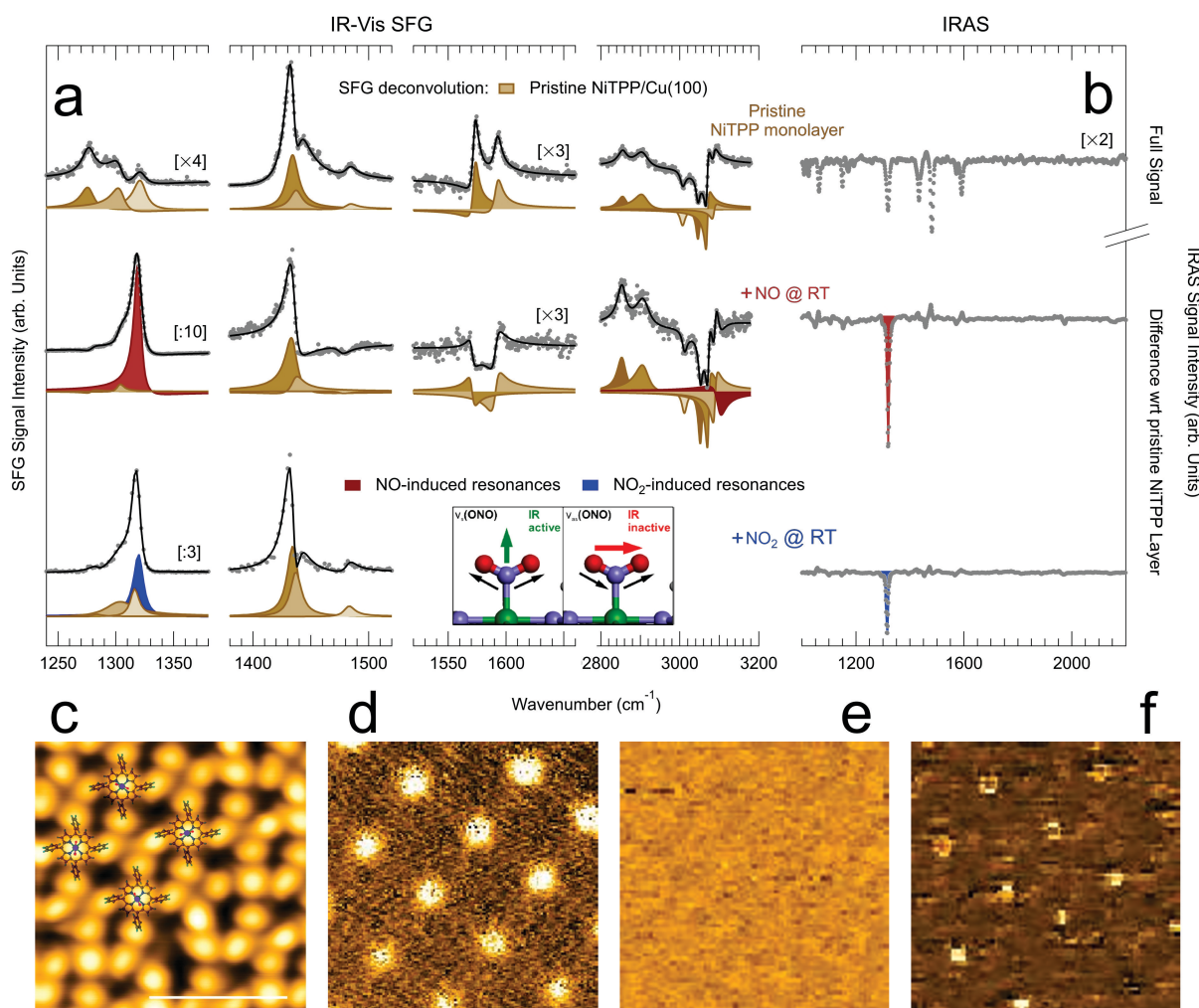
Figure 1. a) IR-Vis SFG spectra of a pristine NiTPP/Cu(100) monolayer at room temperature before (top) and after exposure to NO (middle) and to NO 2 (bottom). For the IR-Vis SFG (IRAS) experiment the layer was exposed to 6 \times 10^2 L ( 5 \times 10^2 L) of NO and to 1 L (1.44 L) of NO 2 , respectively. Data are shown (grey markers) together with the best fit (black lines) and deconvolution (filled profiles) obtained according to the lineshape described in the Supporting Information. b) IRAS spectra corresponding to the IR-Vis SFG spectra in (a). c) Constant-height topographic STM image of the NiTPP/Cu(100) after saturation with NO with superimposed NiTPP models (bias +140 mV; bar corresponds to 2 nm). d–f) Inelastic electron tunneling d 2 I/dV 2 maps at constant height of the same zone in (c) collected at 20, 140, and 170 mV bias, respectively.
